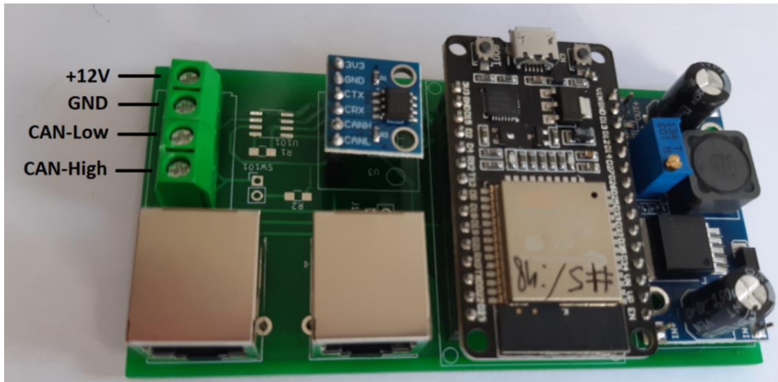
Example of a board with an additional screw connector:
